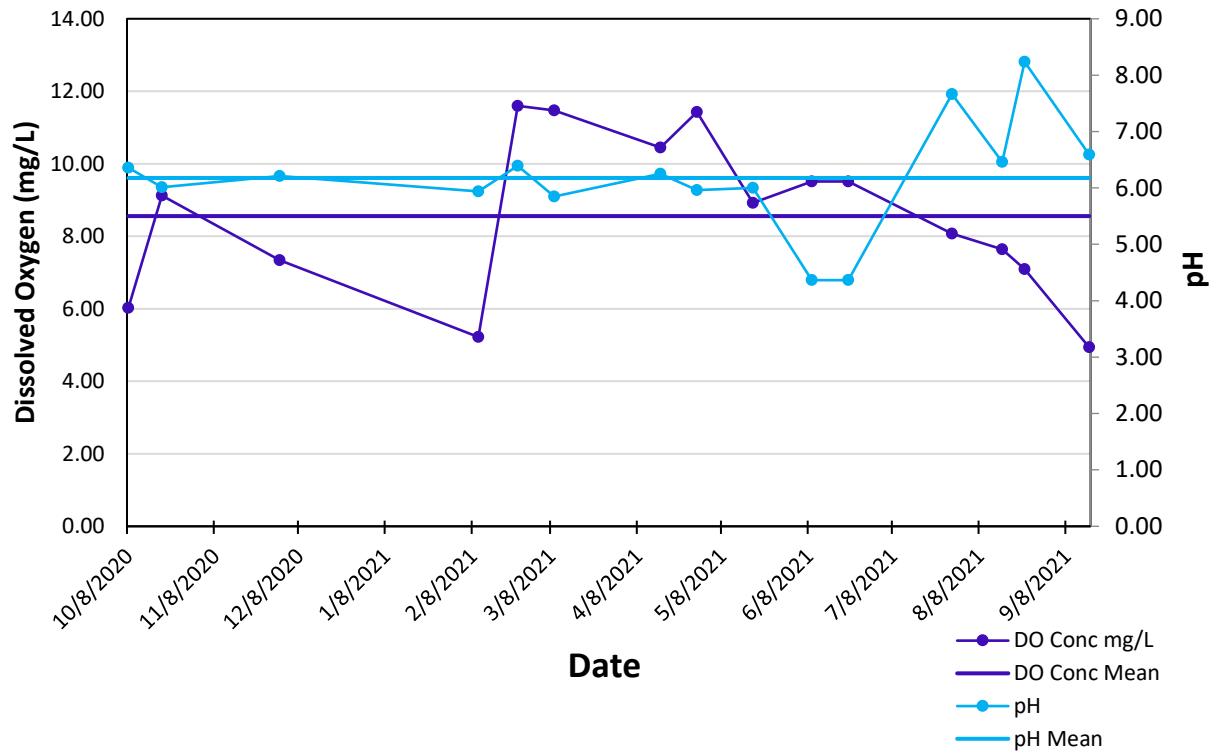
Reservation Wetland Well 2 Average Dissolved Oxygen & pH
