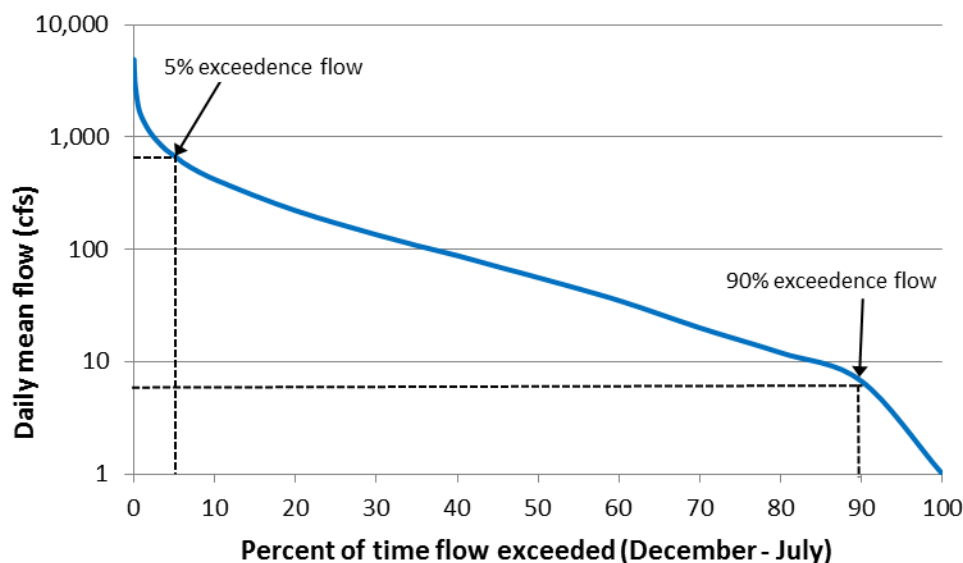
Figure 3-4. Example flow duration curve used to estimate fish migration flows. Data from Bull Creek, 1961–2003 (USGS gage 11476600).
