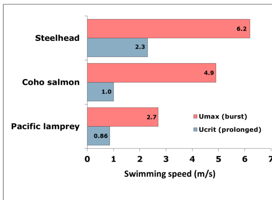
Figure 2-1. Reported swimming speeds of anadromous salmonids (Bell 1990, Lee et al. 2003) and Pacific lamprey (Keefer et al. 2010, Mesa et al. 2003).
